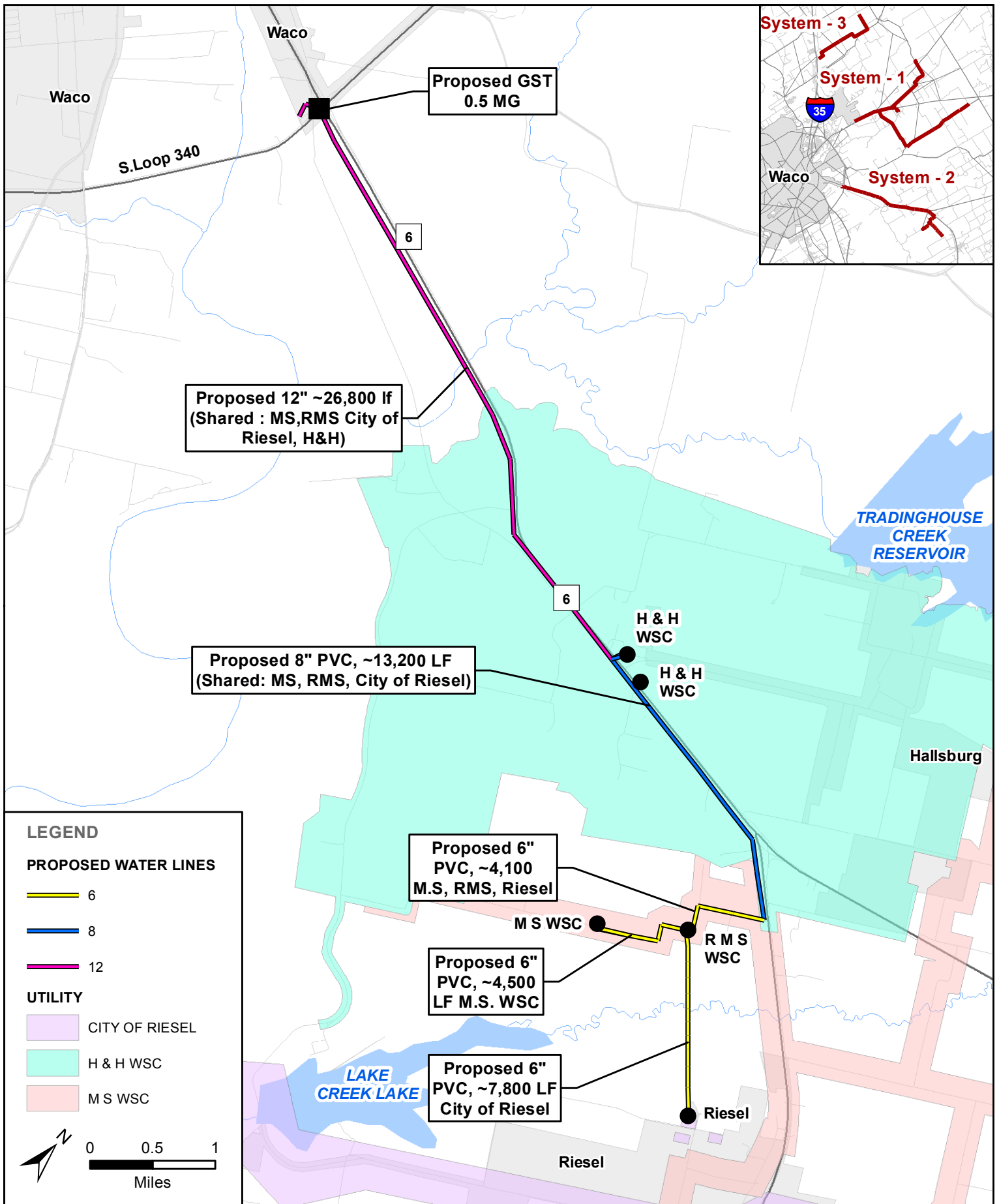
PROPOSED LAYOUT ARSENIC MITIGATION ALT. A: MS- RMS- CITY OF RIESEL- H&H ALTERNATE SUPPLY: CITY OF WACO SW SYSTEM 2
